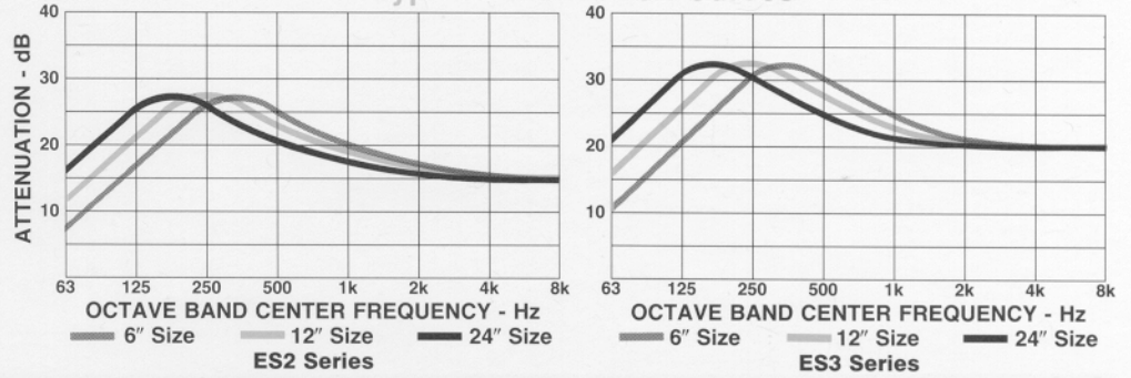
Typical Attenuation Curves
