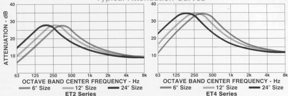
Typical Attenuation Curves
