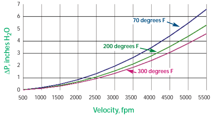
PRESSURE DROP
