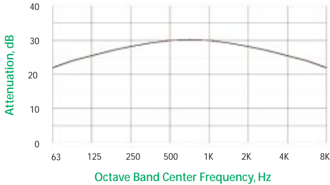
ATTENUATION CURVE, TYPICAL
